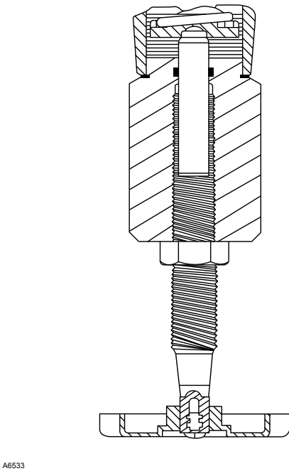
Figure 9. Type 61L (Low Pressure) Handwheel
