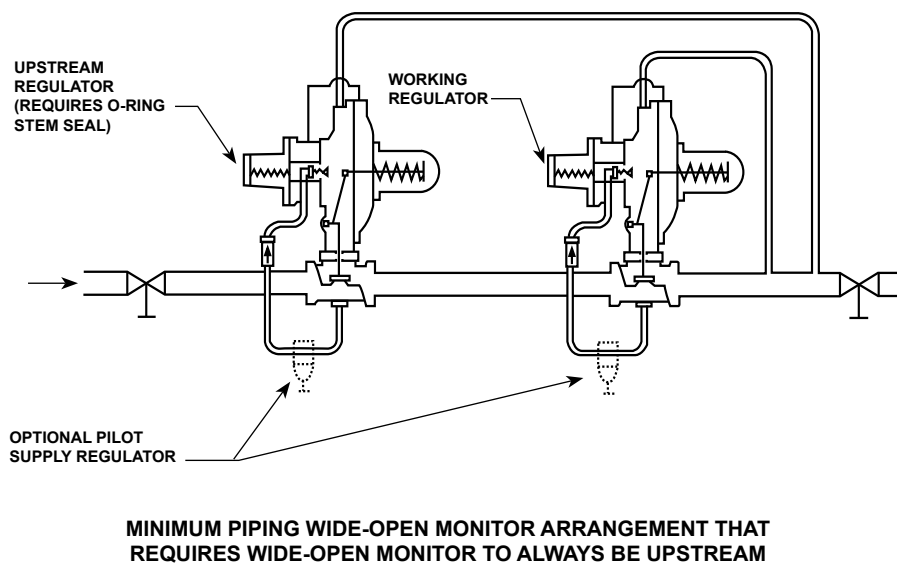
Figure 11. Typical Wide-Open Monitor Installations
