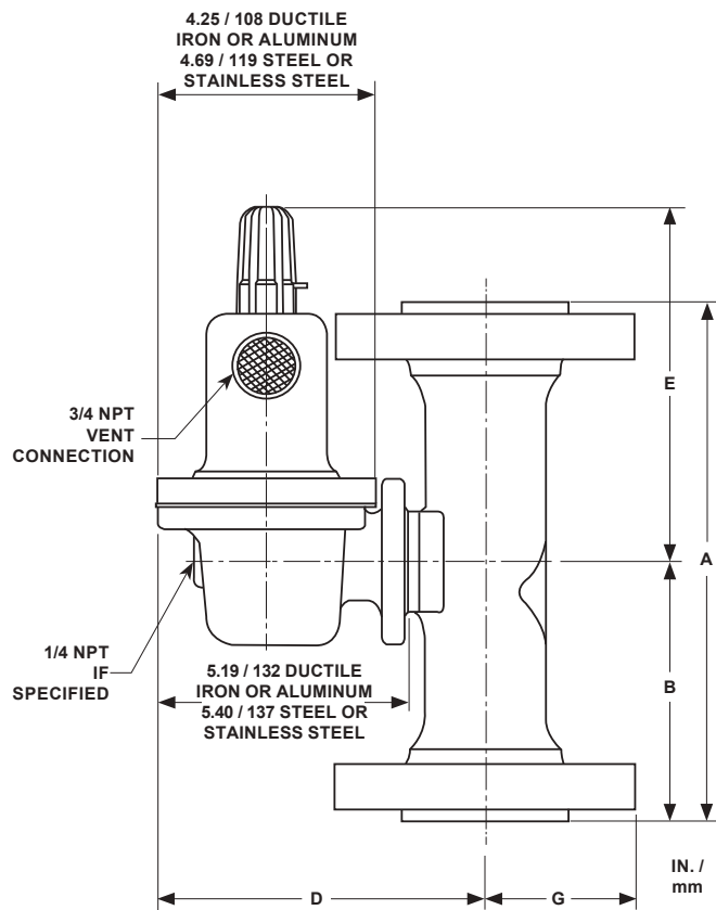
Figure 16. Flanged Dimensions
