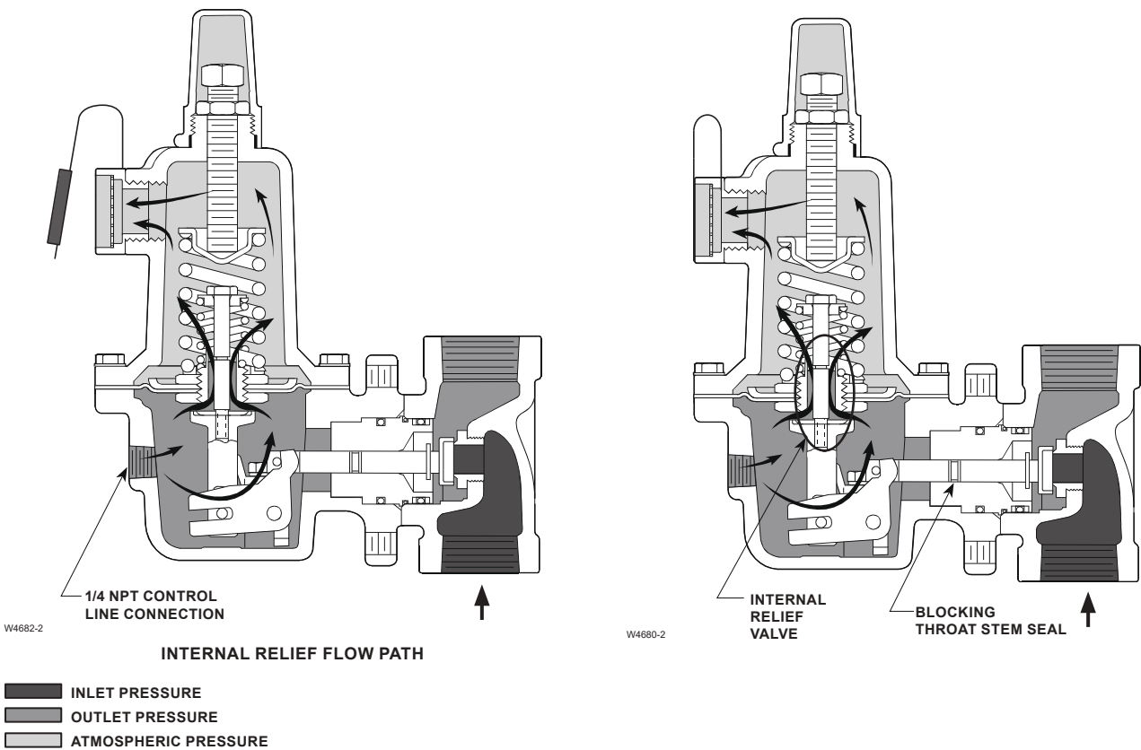
Figure 5. Type 627MR Operational Schematics
