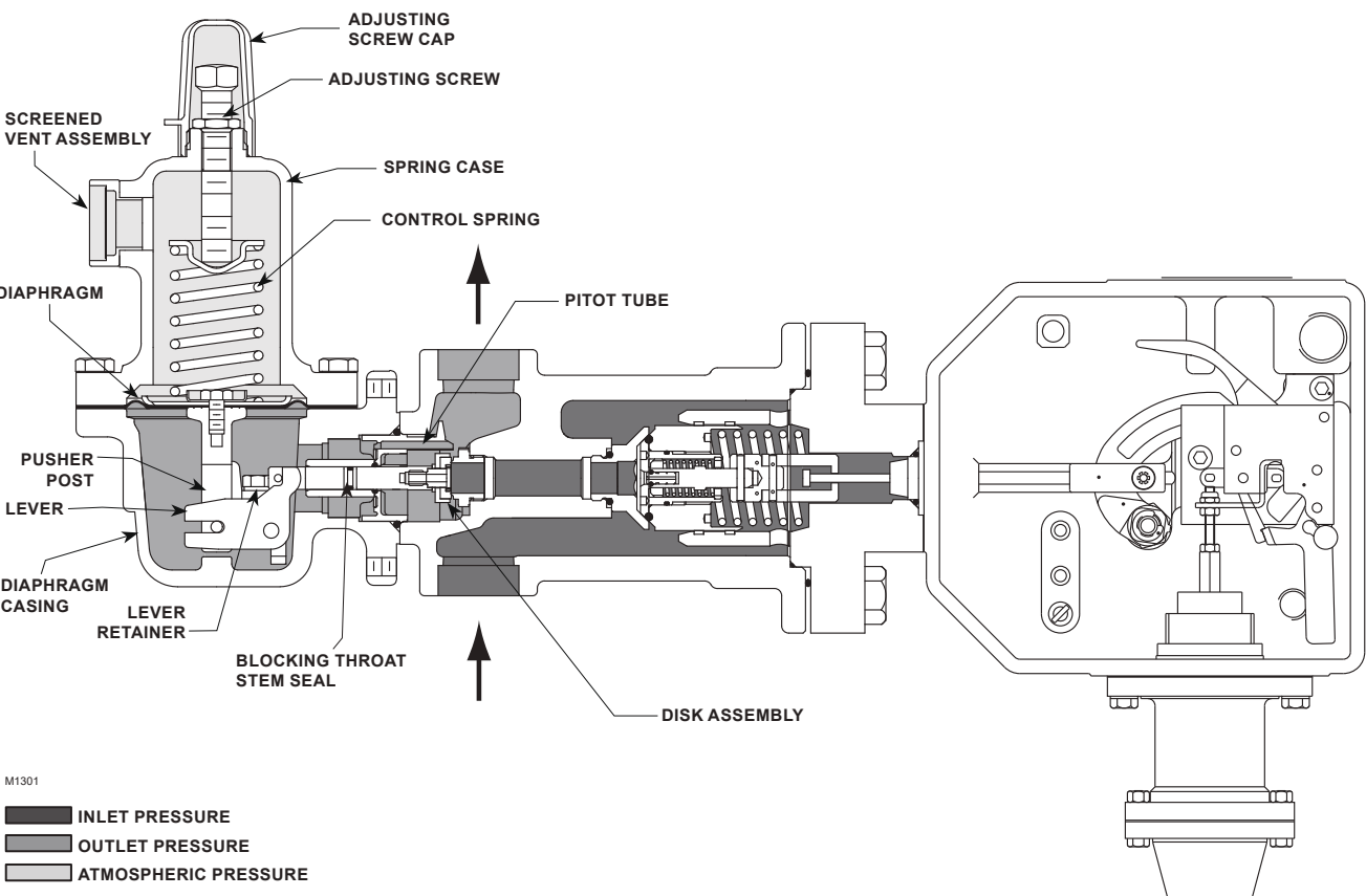
Figure 9. Type 627OSX with Type 627 Regulator and Type OSE Slam-Shut Valve
